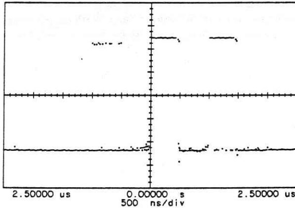
Figure 6-3. Two-Burst Pulse
