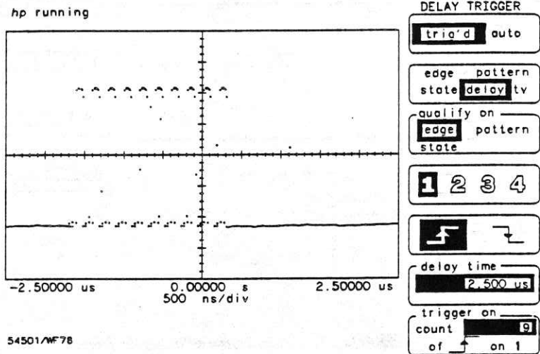
Figure 6-16. Ten Burst Pulse Triggered on Pulse 9
