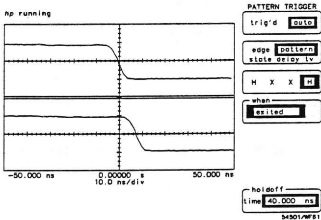
Figure 6-8. HXXX when exited Pattern
