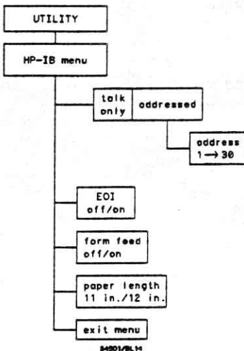
Figure 12-2. HP-IB Menu
