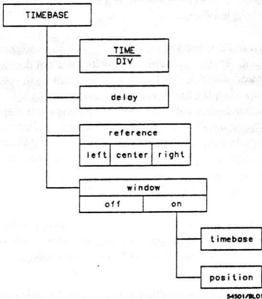
Figure 4-1. Timebase Menu.
