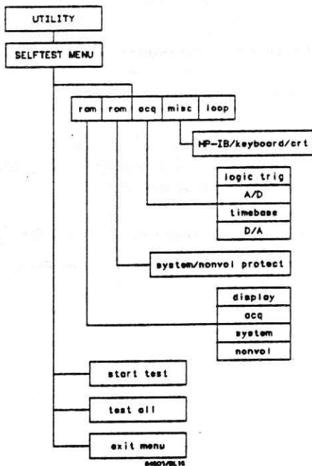
Figure 12-3. Self-Test Menu
