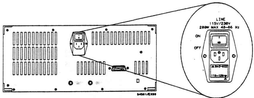
Figure 2-5. Line Switch
