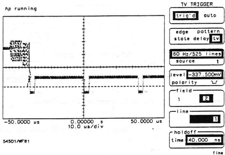
Figure 6-20. Trigger on Field 2, Line 1
