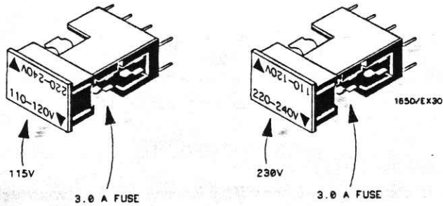
Figure 2-4. Checking for the Correct Fuse
