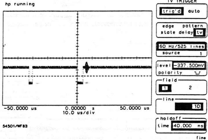
Figure 6-18. Trigger on Field 1, Line 10
