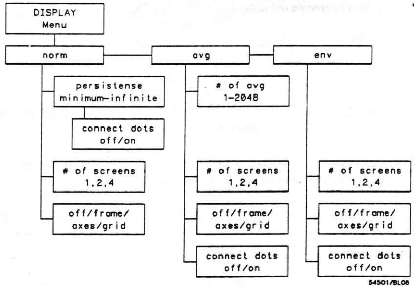
Figure 7-1. Display Menu
