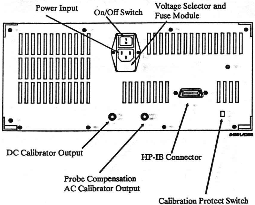
Figure 2-1. Rear Panel Layout
